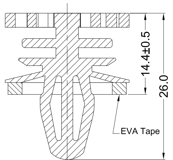
Assembly
